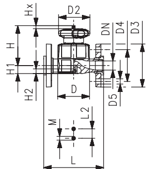
Type 517 Flanged
